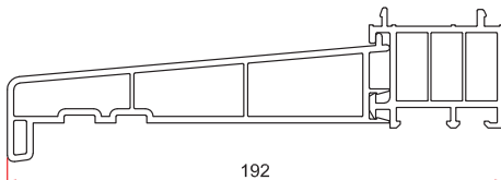
148mm cill 710303 End cap 709151
