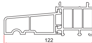
78mm cill 710305 End cap 709153
